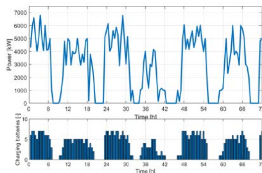
Figure 10: Power consumption (upper graph) and charging batteries (lower graph) at LGAV with 1,000 kW chargers. Weekend case.
